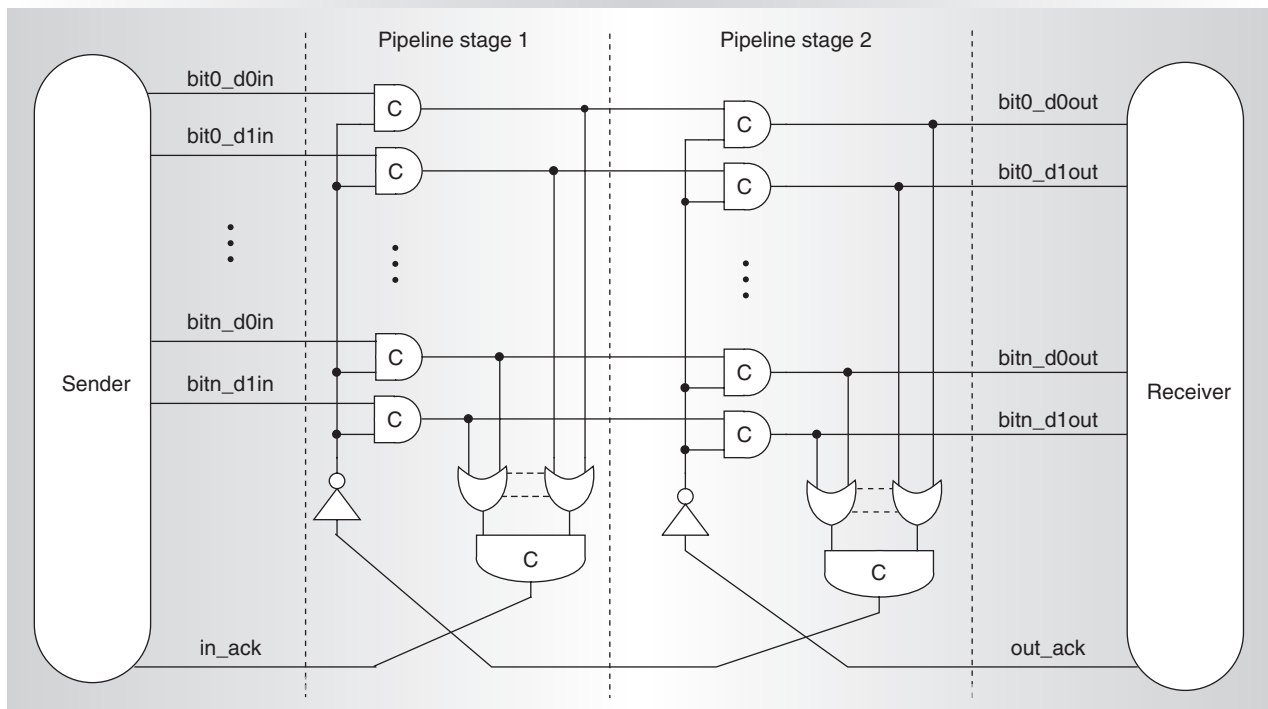
Figure A. Dual-rail, self-timed pipeline channel.
