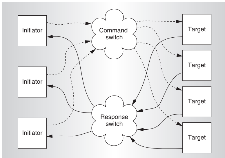
Figure 3. Chain's on-chip network connectivity.
