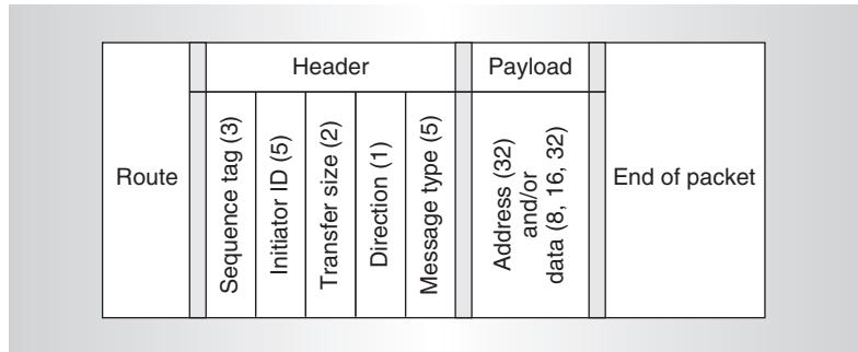
Figure 4. Message format (number of bits shown in parentheses).
