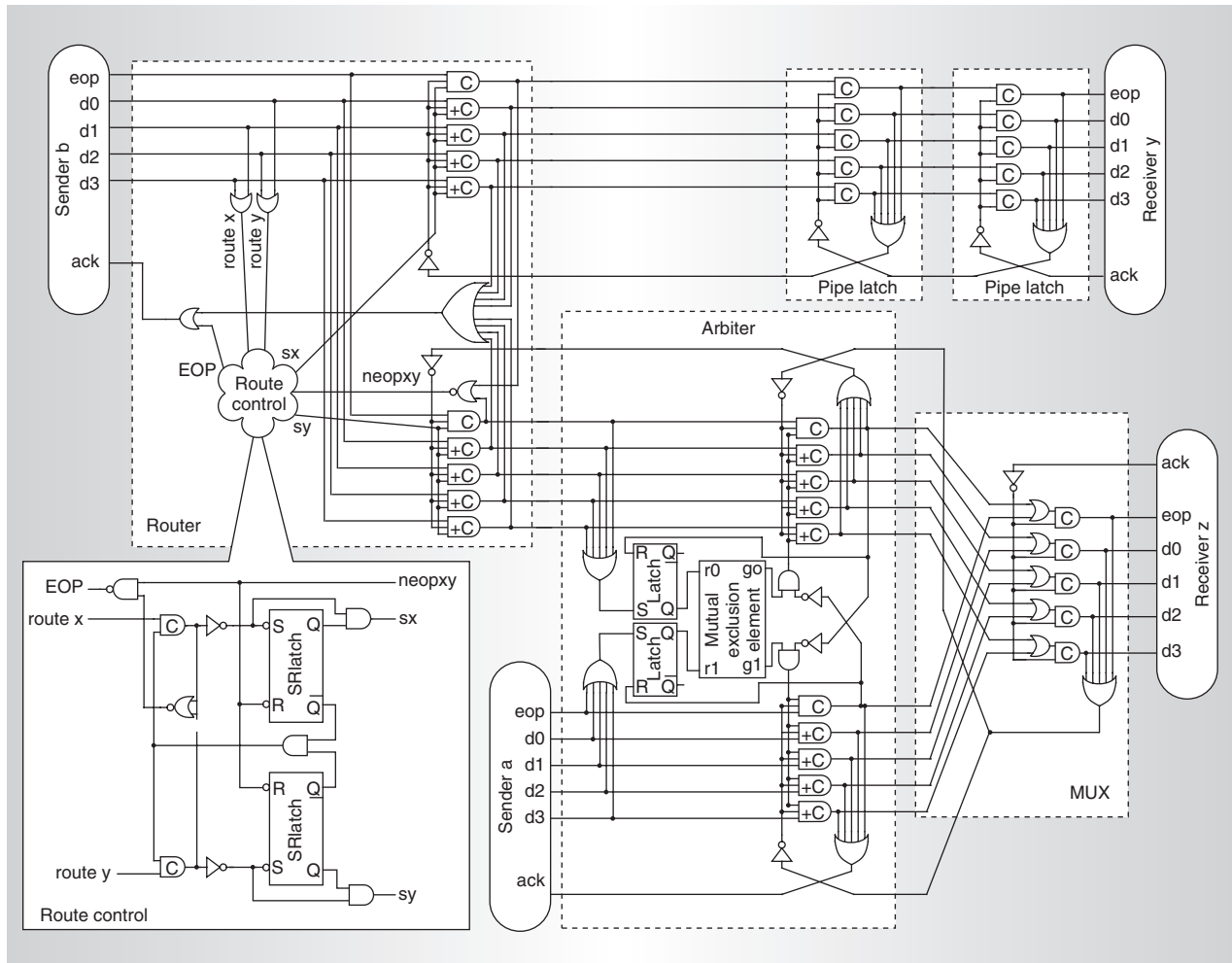
Figure 1. Collage of Chain network components.
